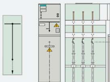
SIMOSEC K
