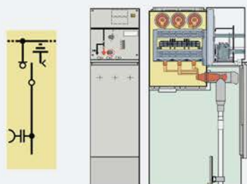
8DJH-R
