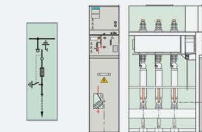
SIMOSEC T
