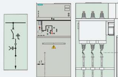
SIMOSEC L1
