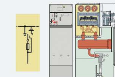
8DJH-T
