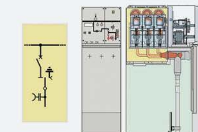
8DJH-L
