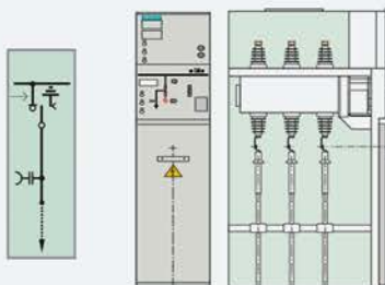
SIMOSEC R
